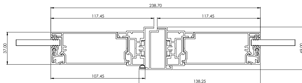
A-08852 FRENCH DOOR LOCKBOX
